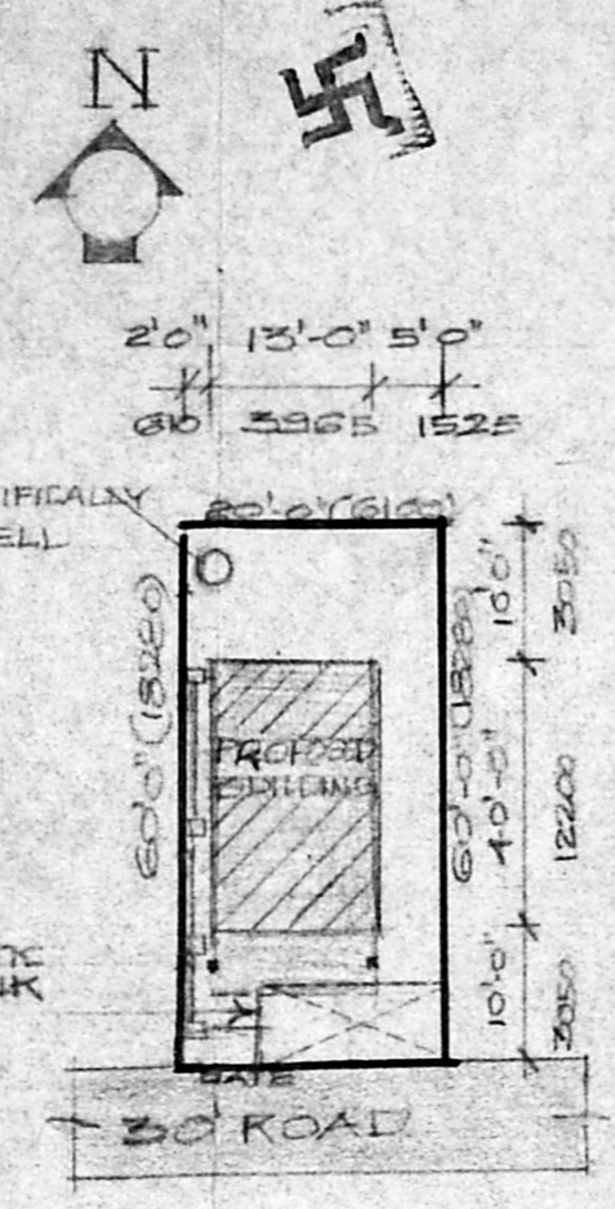
SITE PLAN SCALE 1" : 16'-0"
