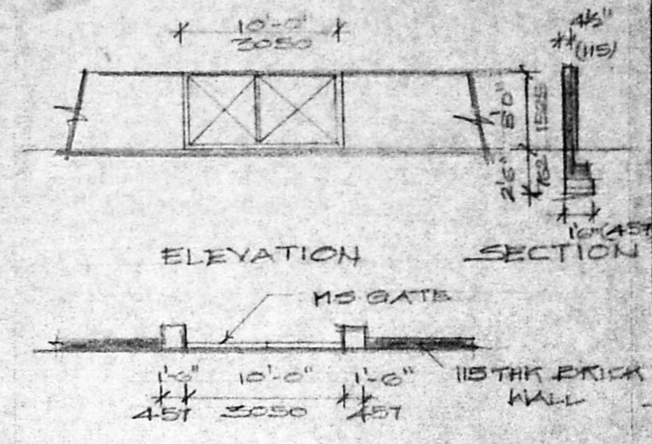
COMPOUND WALL & GATE DETAIL PLAN
