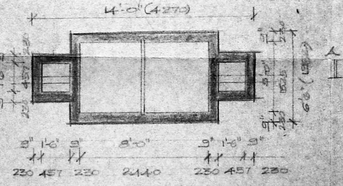
PLAN OF SEPTIC TANK
